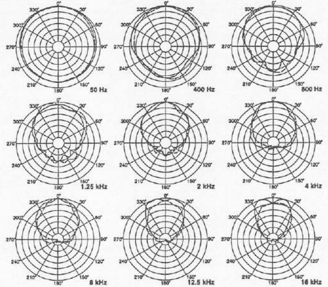
FIGURE 4 — Sx200a Polar Response (anechoic environment)
